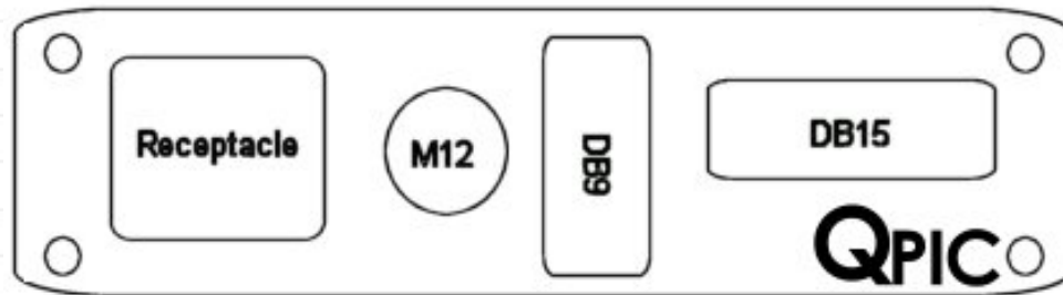
Part# - 24S-CFO Single Receptacle, DB9 Male-Male DB15 Female-Female, DeviceNet M12 Female-Male
