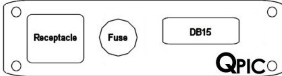
Part# - 24S1-F Single Receptacle, Circuit Breaker, DB15 Female-Female
