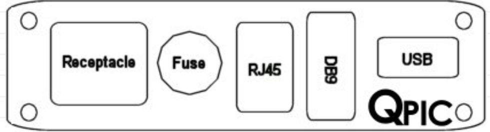
Part# - 24S1-ACM Single Receptacle, Circuit Breaker, RJ45 Female-Female, DB9 Male-Male, USB Female-Female
