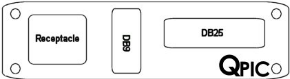
Part# - 24S-BE Single Receptacle, DB9 Female-Female DB25 Male-Male
