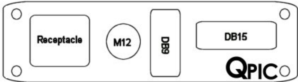
Part# - 24S-BGO Single Receptacle, DB9 Female-Female DB15 Male-Male, DeviceNet M12 Female-Male
