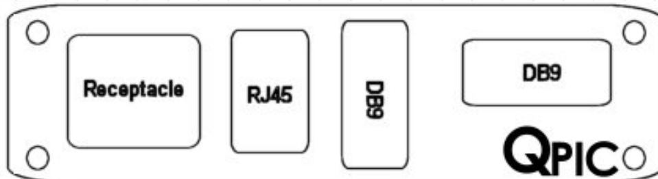
Part# - 24S-ABB Single Receptacle, RJ45 Female-Female DB9 Female-Female, DB9 Female-Female
