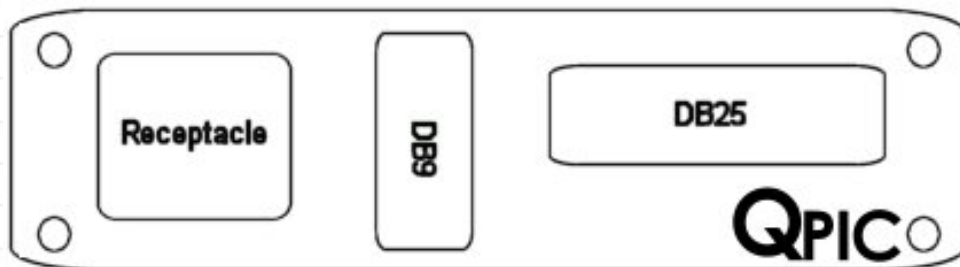
Part# - 24S-CD Single Receptacle, DB9 Male-Male DB25 Female-Female
