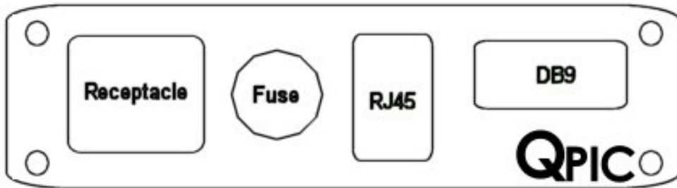
Part# - 24S1-AB Single Receptacle, Circuit Breaker, RJ45 Female-Female, DB9 Female-Female
