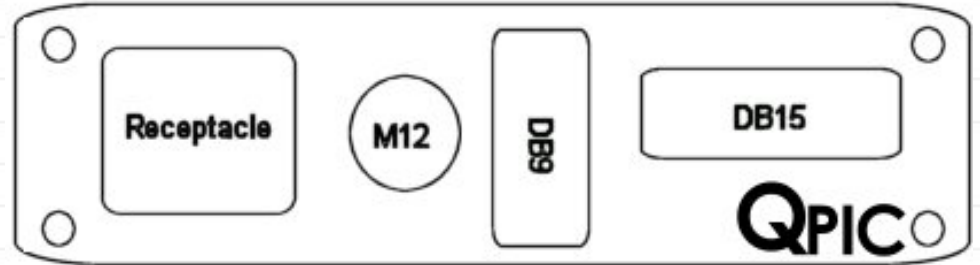
Part# - 24S-BFO Single Receptacle, DB9 Female-Female DB15 Female-Female, DeviceNet M12 Female-Male
