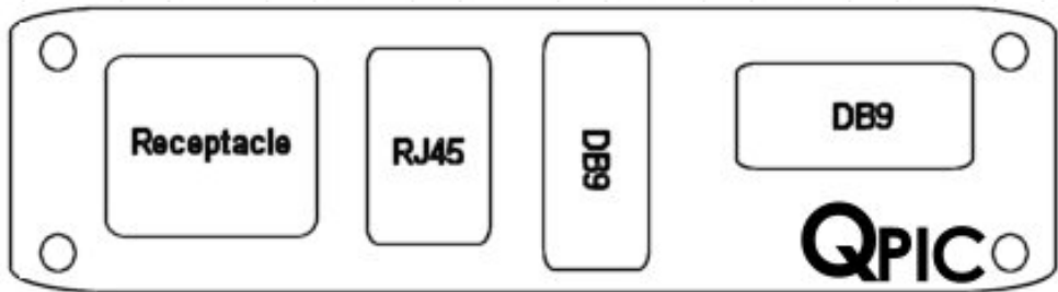
Part# - 24S-ACN Single Receptacle, RJ45 Female-Female DB9 Male-Male, Data Highway DB9 Female-3 Pin Terminal Block
