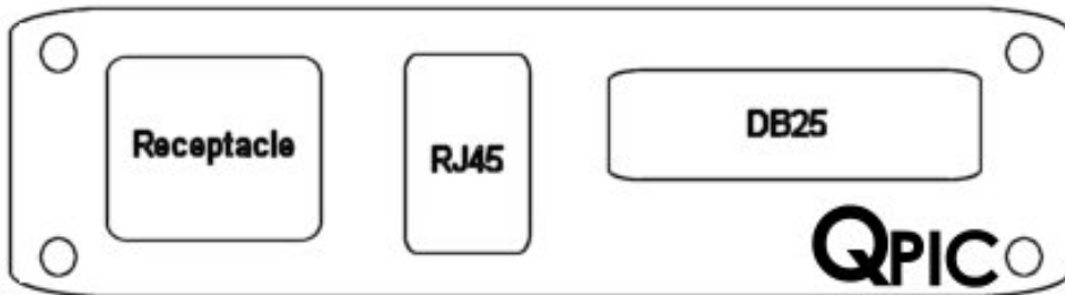
Part# - 24S-AD Single Receptacle, RJ45 Female-Female DB25 Female-Female
