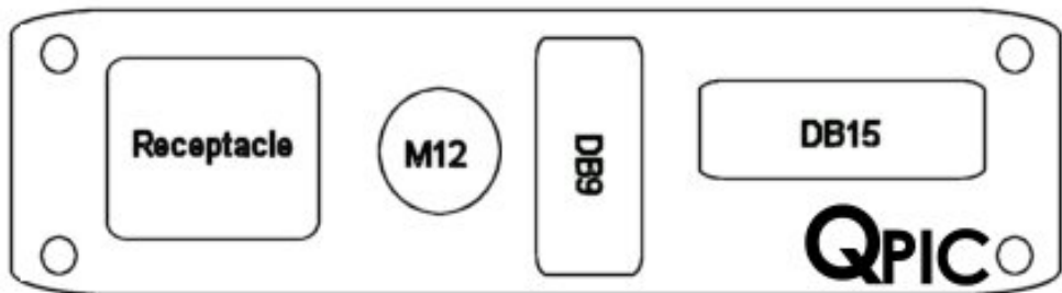
Part# - 24S-CGO Single Receptacle, DB9 Male-Male DB15 Male-Male, DeviceNet M12 Female-Male
