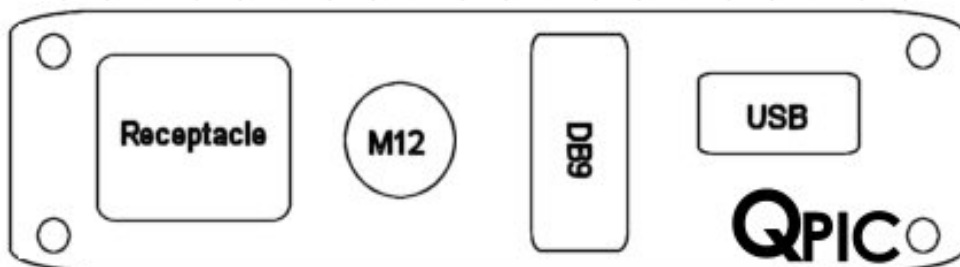
Part# - 24S-CMO Single Receptacle, DB9 Male-Male USB Female-Female, DeviceNet M12 Female-Male
