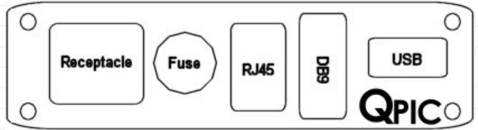
Part# - 24S1-ABM Single Receptacle, Circuit Breaker, RJ45 Female-Female, DB9 Female-Female, USB Female-Female
