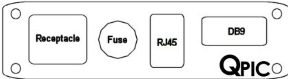
Part# - 24S1-AN Single Receptacle, Circuit Breaker, RJ45 Female-Female, Data Highway DB9 Female-3 Pin Terminal Block
