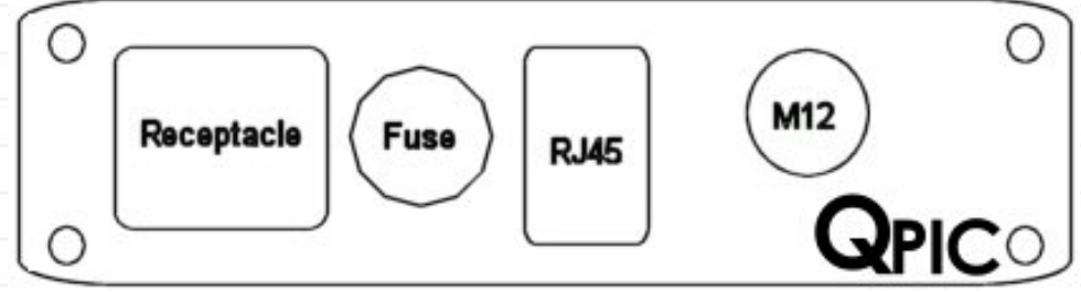
Part# - 24S1-AO Single Receptacle, Circuit Breaker, RJ45 Female-Female, DeviceNet M12 Female-Male
