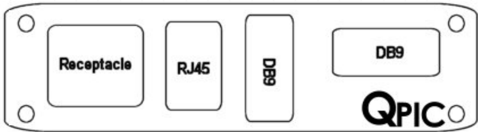
Part# - 24S-ABN Single Receptacle, RJ45 Female-Female DB9 Female-Female, Data Highway DB9 Female-3 Pin Terminal Block
