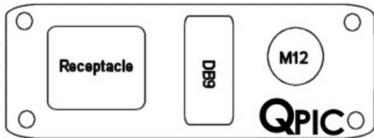
Part# - 16S-BO Single Receptacle, DB9 Female-Female, DeviceNet M12 Female-Male
