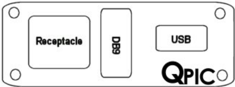
Part# - 16S-CM Single Receptacle, DB9 Male-Male, USB Female-Female
