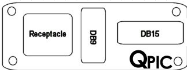
Part# - 16S-CF Single Receptacle, DB9 Male-Male, DB15 Female-Female
